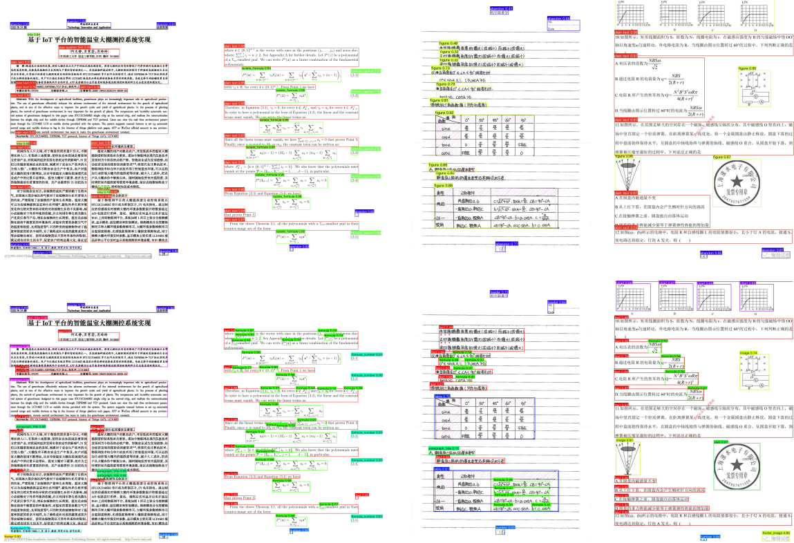
Figure 3. Comparison of our results and DocLayout-YOLO [14].
